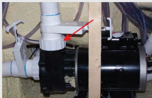
FIGURE 1.9b : PUMP UNION; LOOSEN UP TO BLEED AIR
